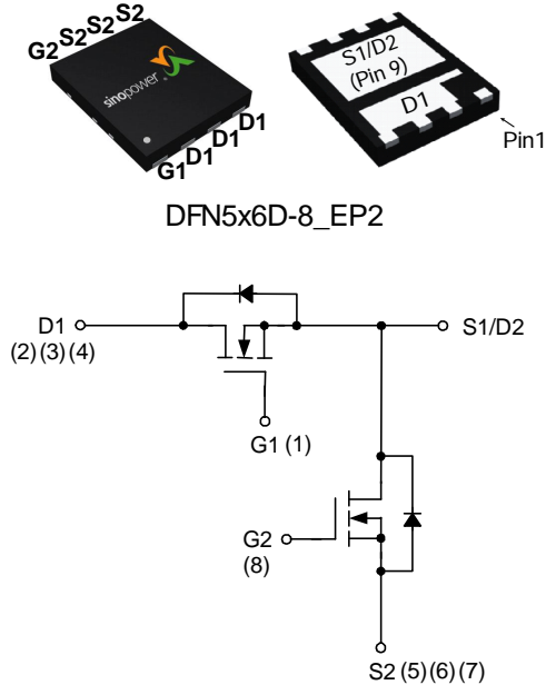
N-Channel MOSFET
